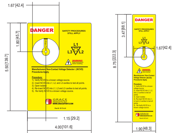
R-T3-LH Horizontal Label Applies to the R-T3
