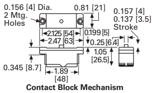
Contact Block Mechanism
