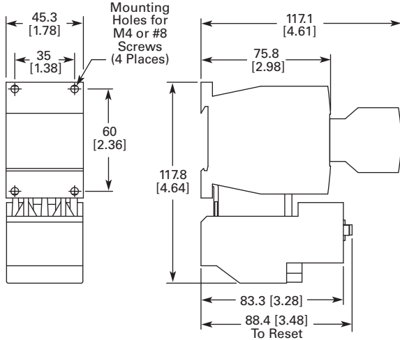
Frame B, XTAE007B–XTAE015B Starters with XTOB (7–12A)
